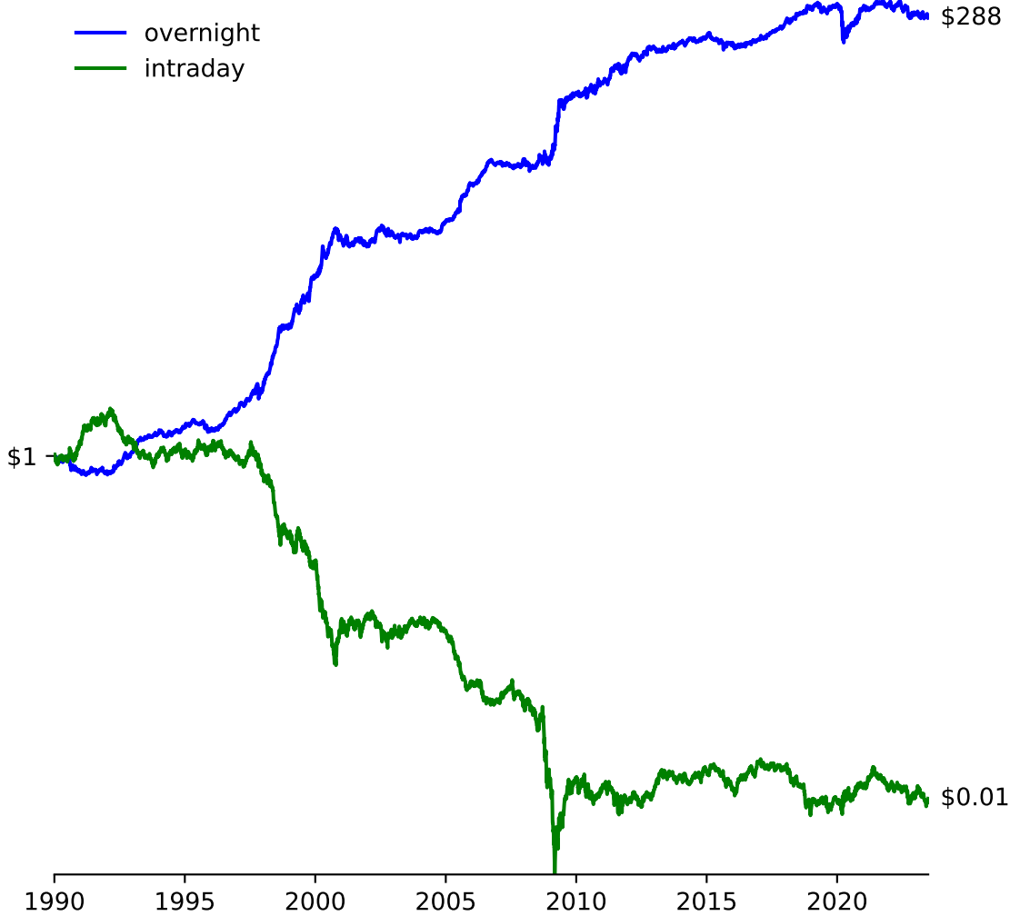
Value of $1 invested in International Paper (IP), getting only overnight or intraday returns (logarithmic vertical scale)
